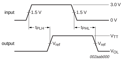
Fig 5. Propagation delay, A port to B port
