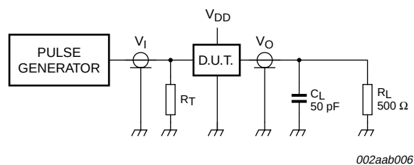
Fig 10. Load circuitry for A outputs
