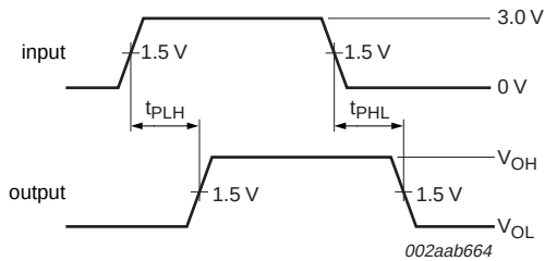
Fig 9. Propagation delay, 1AI to AO2
